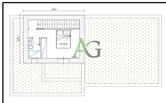
FLOOR PLAN FIRST FLOOR
